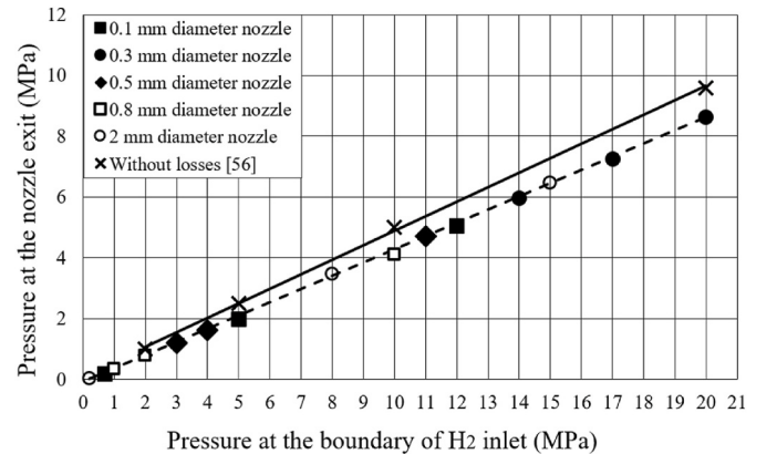
Fig. 2. Variation of the pressure at the nozzle exits with pressure at the boundary position. The solid black line is fitted to predicted data using analytical equation without losses [56], dashed black line is a fitted curve to simulation results considering losses.
