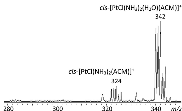
Fig. 1. ESI mass spectrum of a cisplatin-ACM solution. The isotope pattern at m/z 322–326 correspond to cis-[PtCl(NH_3)_2(ACM)]^+ , while cis-[PtCl(NH_3)_2(H_2O)(ACM)]^+ accounts for the isotope pattern at m/z 340–344.
