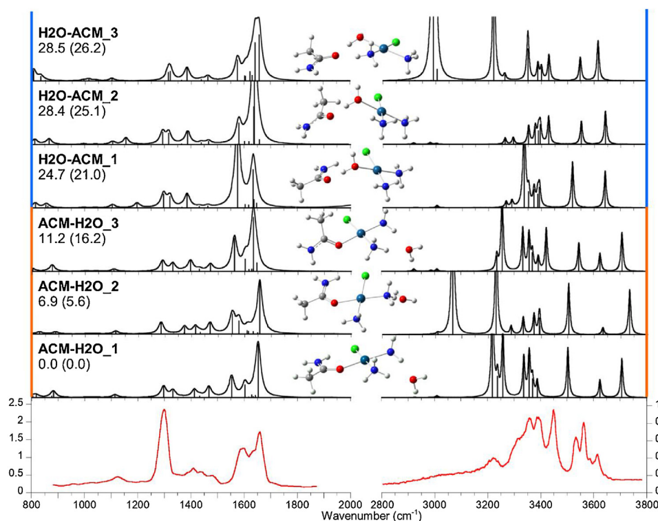
Fig. 5. IRMPD spectrum of \text{cis-[PtCl(NH}_3)_2(\text{H}_2\text{O})(\text{ACM})]^+ (red profile) compared with the theoretical IR spectra of ACM-H2O_1 , ACM-H2O_2 , ACM-H2O_3 , H2O-ACM_1 , H2O-ACM_2 and H2O-ACM_3 . Optimized geometries at the B3LYP/6-311+G(d,p) level are reported together with relative free energies at the \omega\text{B97X-D} and B3LYP (in bracket) levels at 298 K in \text{kJ mol}^{-1} .
