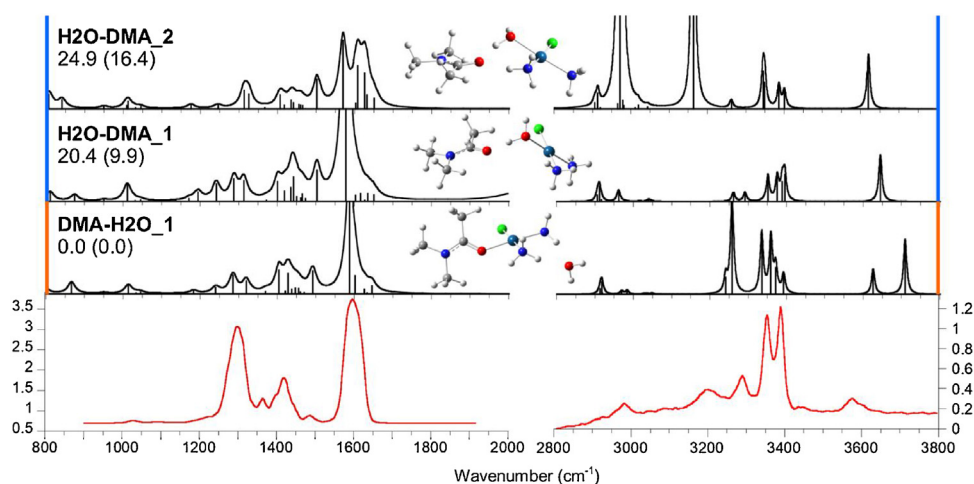
Fig. 6. IRMPD spectrum of \text{cis-[PtCl(NH}_3)_2(\text{H}_2\text{O})(\text{DMA})]^+ (red profile) compared with the theoretical IR spectra of DMA-H2O_1 , H2O-DMA_1 and H2O-DMA_2 . Optimized geometries at the B3LYP/6-311+G(d,p) level are reported together with relative free energies at the \omega\text{B97X-D} and B3LYP (in bracket) levels at 298 K in \text{kJ mol}^{-1} .
