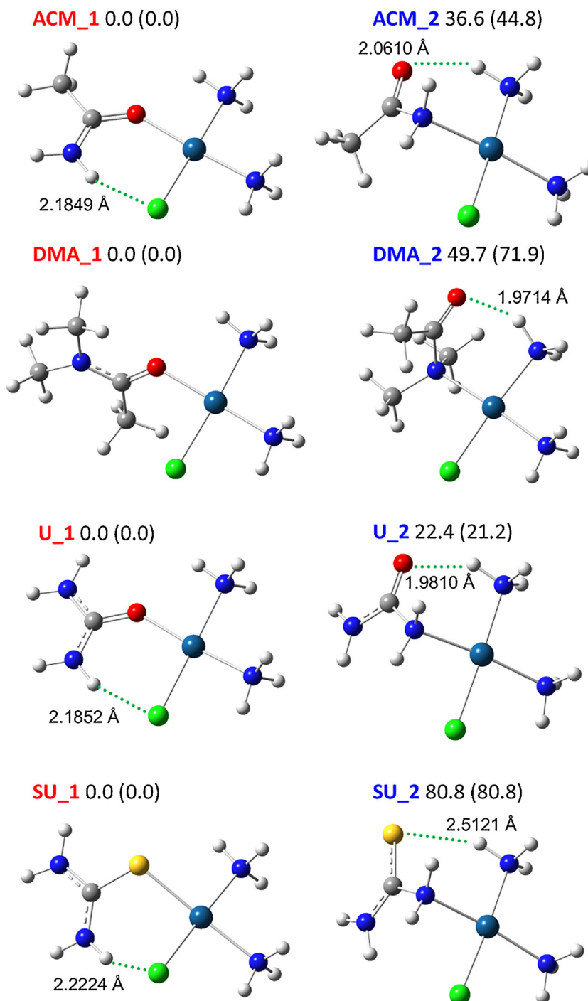
Fig. 3. Optimized geometries of \text{cis-}[\text{PtCl}(\text{NH}_3)_2(\text{L})]^+ complexes at B3LYP/6-311+G(d,p) (LanL2TZ for Pt) level of theory. Relative free energies as calculated at the \omega\text{B97X-D} and B3LYP (in brackets) level at 298 K are given in \text{kJ mol}^{-1} .
