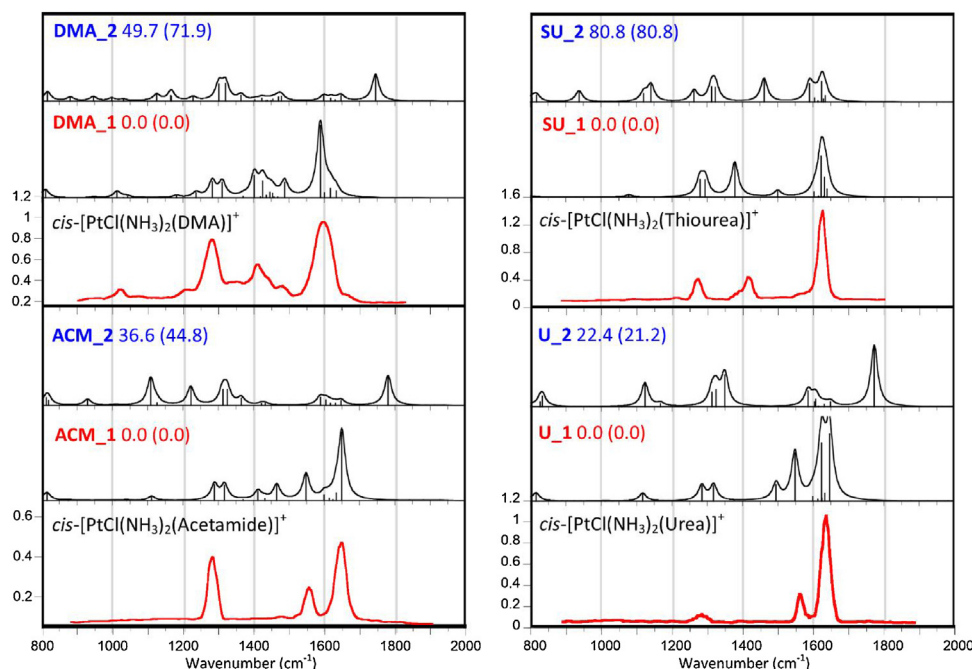
Fig. 4. IRMPD spectra (red profiles) of cis\text{-[PtCl(NH}_3)_2\text{(L)]}^+ ( L = \text{ACM, DMA, U, TU} ) compared with the IR spectra (black profiles) calculated at B3LYP/6-311+G(d,p) level for the isomers reported in Fig. 3. Theoretical harmonic frequencies are scaled by a factor of 0.974. Relative free energies at 298 K are in kJ mol -1 , as calculated at the \omega\text{B97X-D} and B3LYP (in brackets) level.
