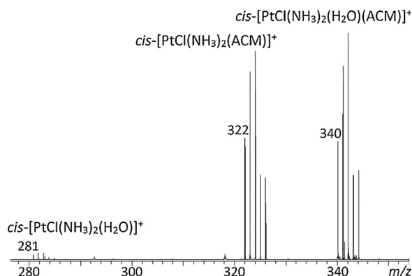
Fig. 2. ESI-MS 2 obtained upon CID of cis-[PtCl(NH_3)_2(H_2O)(ACM)]^+ at m/z 340. The two observed fragmentation channels correspond to water loss ( m/z 322) and ACM loss ( m/z 281).
