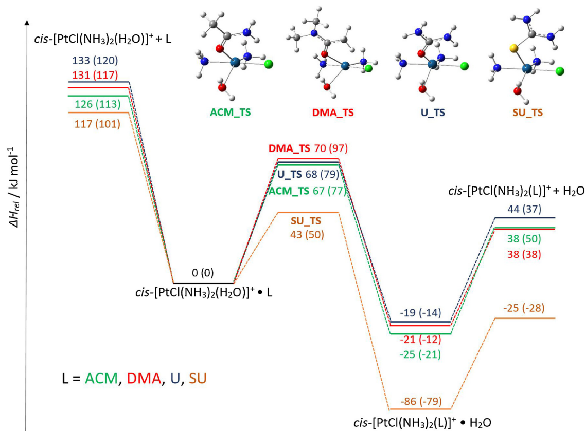
Fig. 8. PES for the reaction of \text{cis-}[\text{PtCl}(\text{NH}_3)_2(\text{H}_2\text{O})]^+ + \text{L} ( \text{L} = \text{ACM, DMA, U} and \text{SU} ). Geometries of the transition states optimized at B3LYP/6-311+G(d,p) are shown. Relative enthalpies ( \text{kJ mol}^{-1} ) are reported at the \omega\text{B97X-D}/6-311+G(d,p) level. Values at B3LYP/6-311+G(d,p) level are also reported (in brackets).
