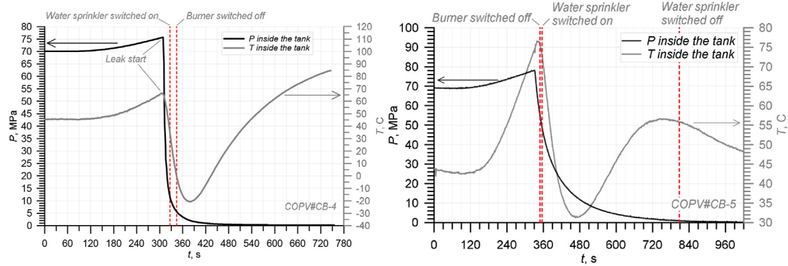
Fig. 7 – Pressure and temperature transients inside \mu LNB tank prototypes during the fire tests: COPV#CB-4 (left) and COPV#CB-5 (right) both with liner L2.
