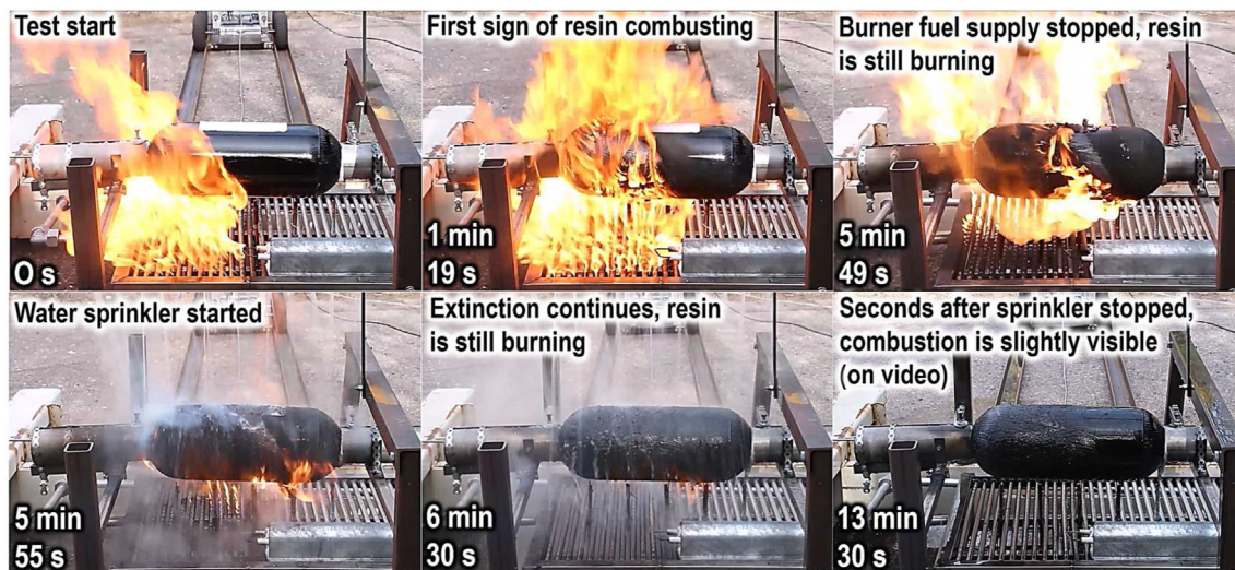
Fig. 8 – Snapshots of the \mu LNB tank prototype COPV#CB-5 behaviour in the fire test.
